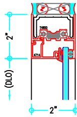
HEAD CONDITION W/O COMP (1/4" GLASS)
