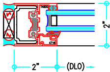
JAMB CONDITION W/O COMP
