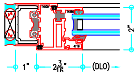
JAMP / VENT CONDITION W/O COMP
