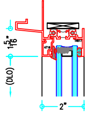
HEAD CONDITION (NAIL FIN)
