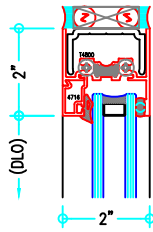
HEAD CONDITION W/O COMP (1" GLASS)
